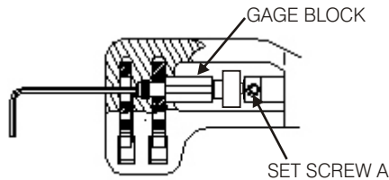
Plunger Tip adjustment Figure 4
