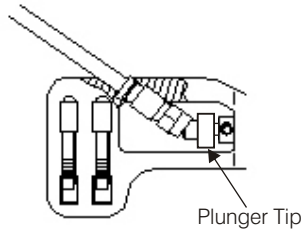
Insert Cable and Connector Figure 1
